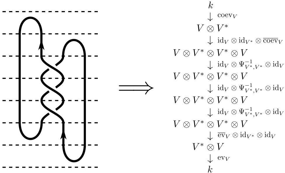
Example computation for the Reshetikhin-Turaev invariants on the trefoil knot.
