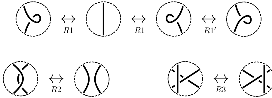
The three Reidemeister moves and weakened first Reidemeister move.
