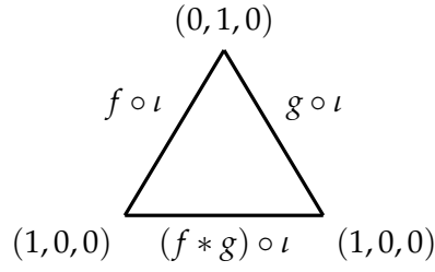
Figure 2.2: The singular simplex \sigma in the proof of Lemma 2.6
