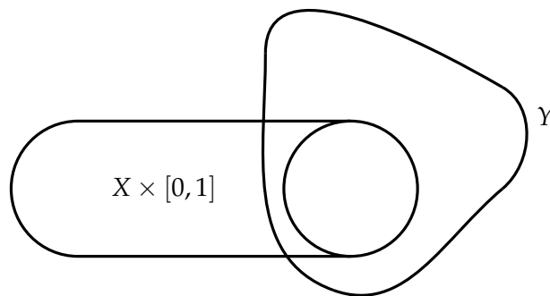
Figure 14.1: The mapping cylinder of f: X \rightarrow Y
