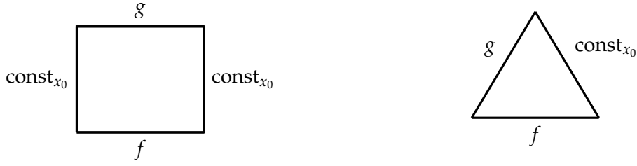
Figure 2.1: The homotopy H and the singular simplex \sigma in the proof of Lemma 2.4
