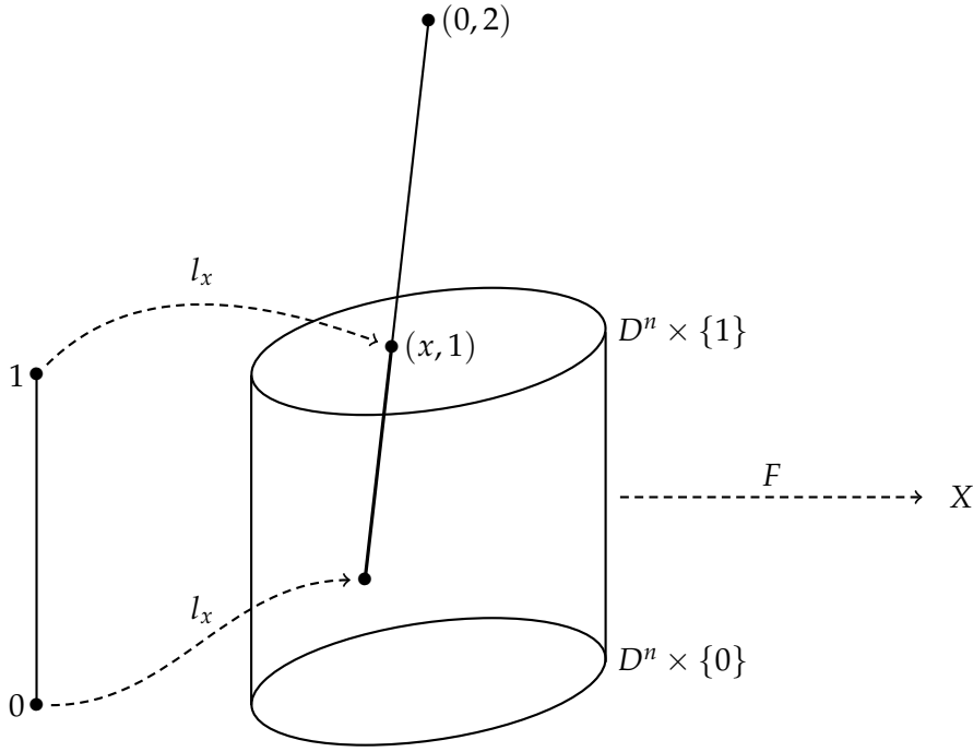
Figure 13.2: Construction of the homotopy H in the proof of Lemma 13.10
