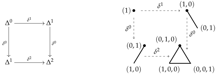
Figure 1.5: The relation \delta^2\delta^0 = \delta^0\delta^1 . The \bullet marks the images of \Delta^0 in \Delta^1 and in \Delta^2 .
